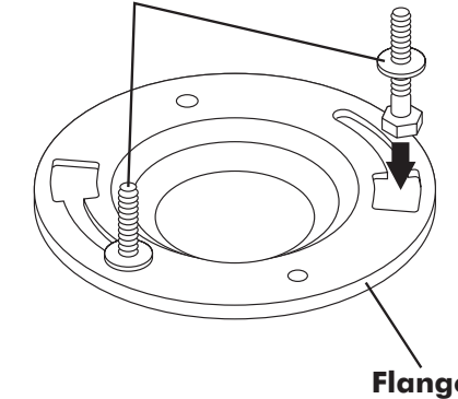
5/16" Diameter bolts
